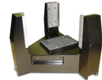
115 lb. base for a nanolithography machine.
